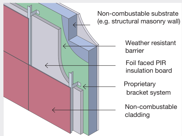
Figure 4: Facade system using foil faced PIR insulation board.
