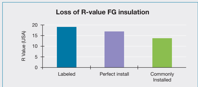
Figure 5: Effect of air leakage on the installed R-value of FG batt insulation.
