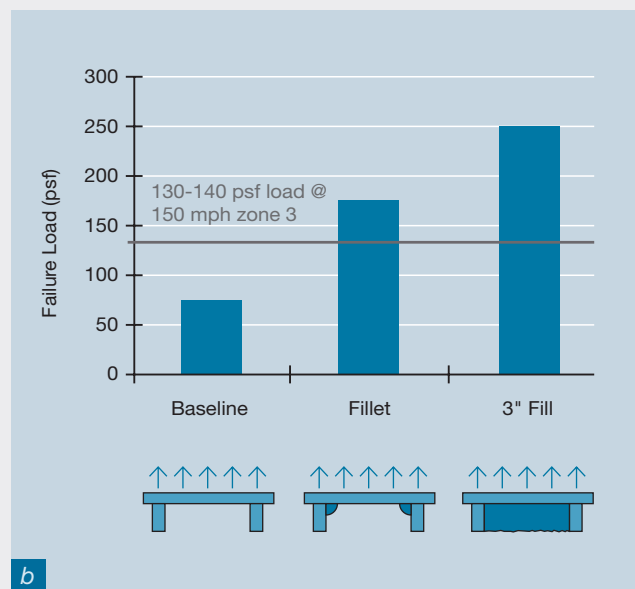
Figure 10: a) Racking strength. 25 b) Wind uplift. 17
